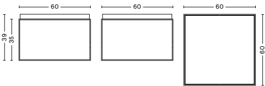
TRAY TABLE COFFEE Length 60 cm Width 60 cm Height 39 cm Weight 10,5 kg
