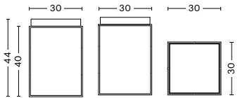
TRAY TABLE S HIGH Length 30 cm Width 30 cm Height 44 cm Weight 4,2 kg
