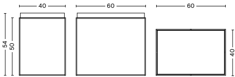
TRAY TABLE L Length 60 cm Width 40 cm Height 54 cm Weight 8,4 kg
