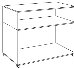
trolley 5 width x depth x height: 860 x 430 x 650 mm white or black
