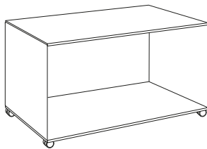
trolley 4 width x depth x height: 860 x 430 x 450 mm white or black
