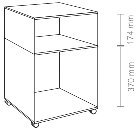
trolley 2 width x depth x height: 430 x 430 x 650 mm white or black
